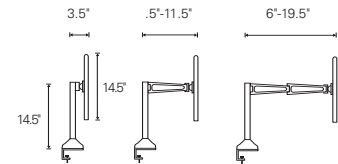
M7 LP Clamp Mount on Slim Post with FEA (Front End Adjuster) with 6" dynamic height adjustment
