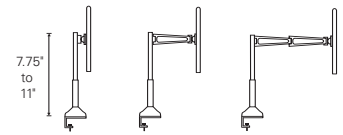
M7 LP Clamp Mount with 3.25" dynamic height adjustment FEA (Front End Adjuster) with 6" dynamic height adjustment
